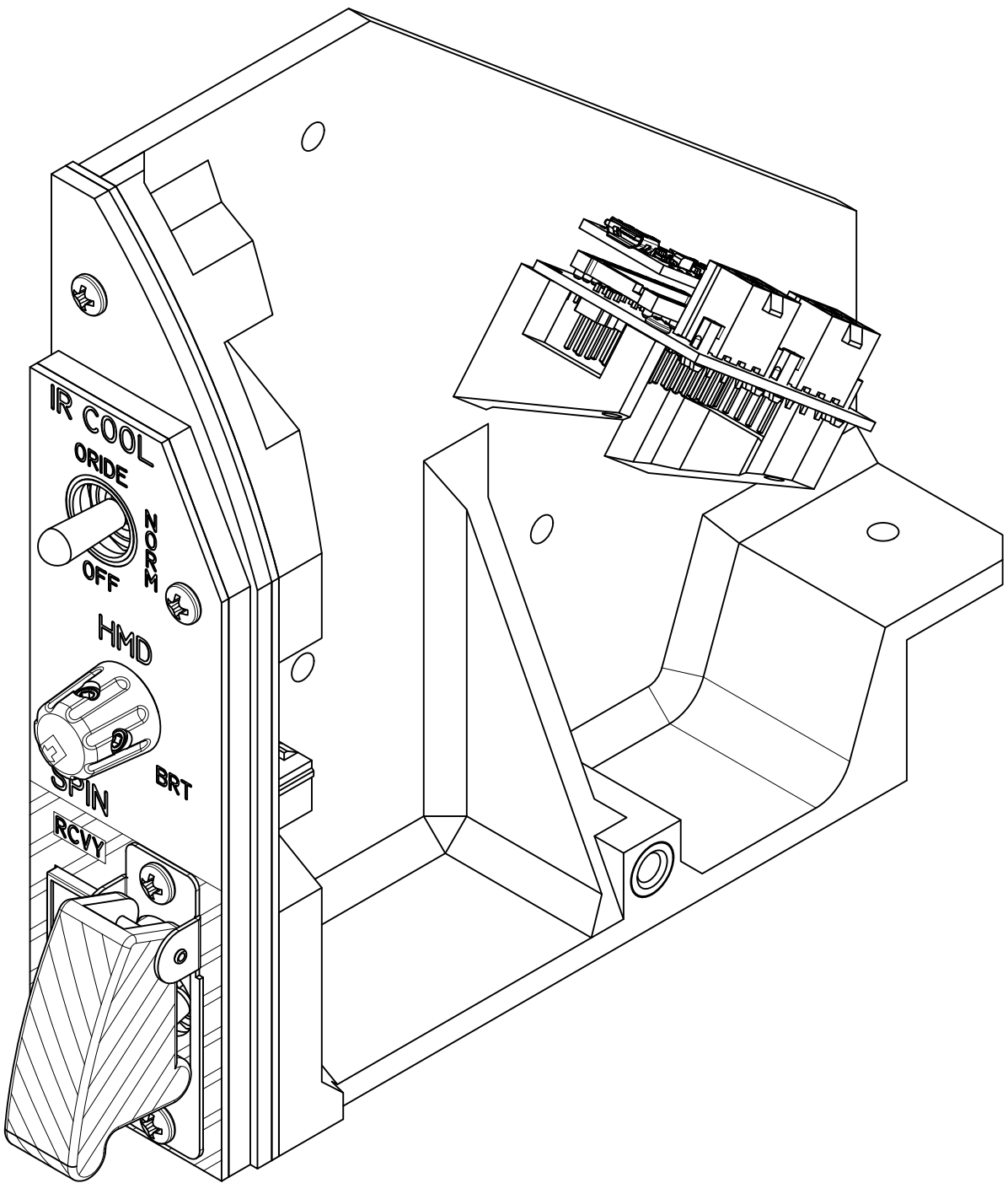
-1 ASSY
